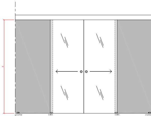
ELEVATION - CLOSED POSITION [VIEW FROM INSIDE OFFICE]
