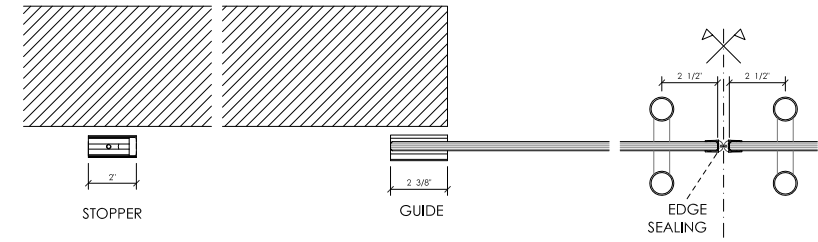
DOOR DETAILS WITH BAR HANDLE - CLOSED POSITION
