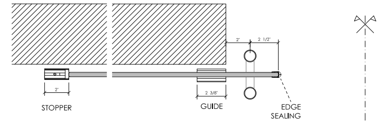
DOOR DETAILS WITH BAR HANDLE - OPENED POSITION
