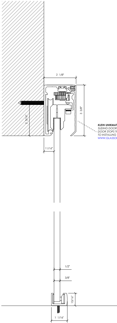
TRACK AT WALL EXPOSED TRACK
