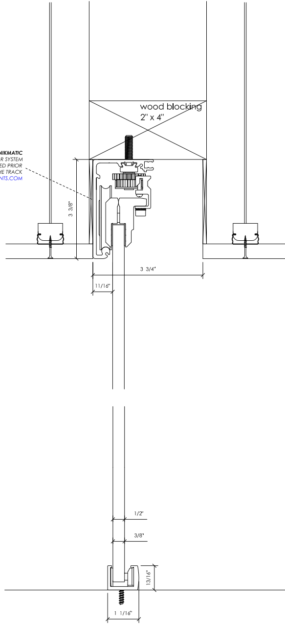
TRACK AT WALL RECESSED TRACK
