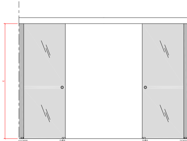
ELEVATION - OPENED POSITION [VIEW FROM INSIDE OFFICE]
