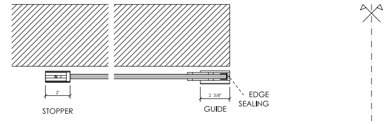
DOOR DETAILS WITH ROUND PULL - OPENED POSITION
