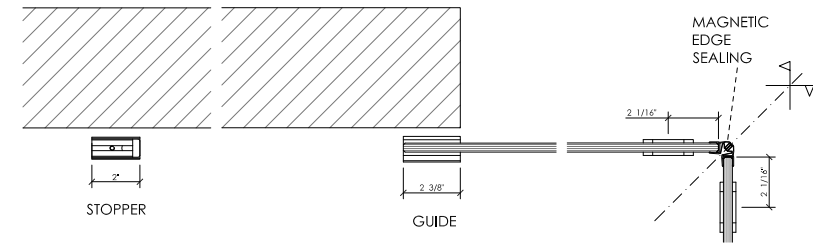
DOOR DETAILS WITH ROUND PULL - OPENED POSITION
