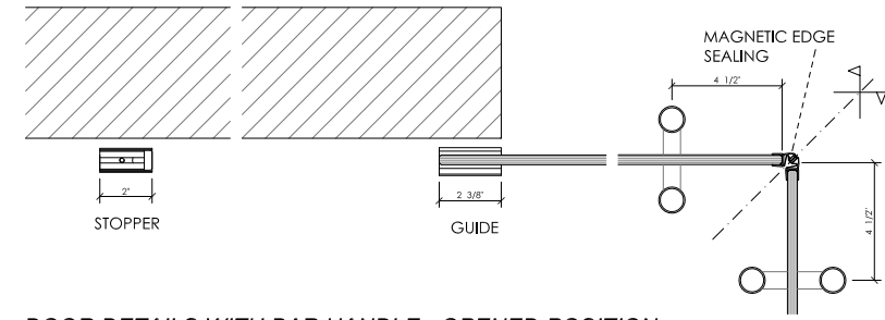
DOOR DETAILS WITH BAR HANDLE - OPENED POSITION
