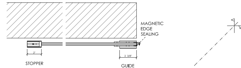
DOOR DETAILS WITH ROUND PULL - OPENED POSITION
