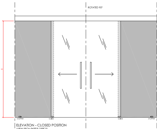
ELEVATION - CLOSED POSITION (VIEW FROM INSIDE OFFICE)
