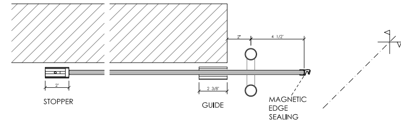
DOOR DETAILS WITH BAR HANDLE - OPENED POSITION
